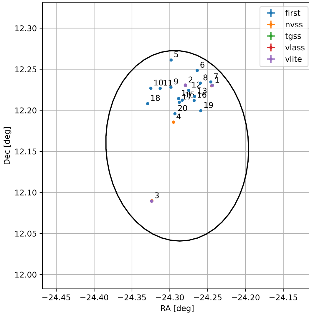
4FGL J2222.8+1209
