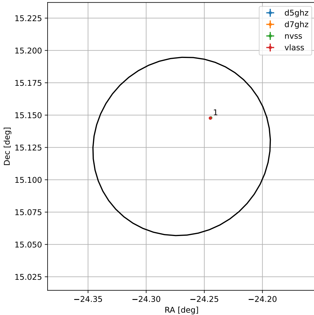
4FGL J2222.9+1507
