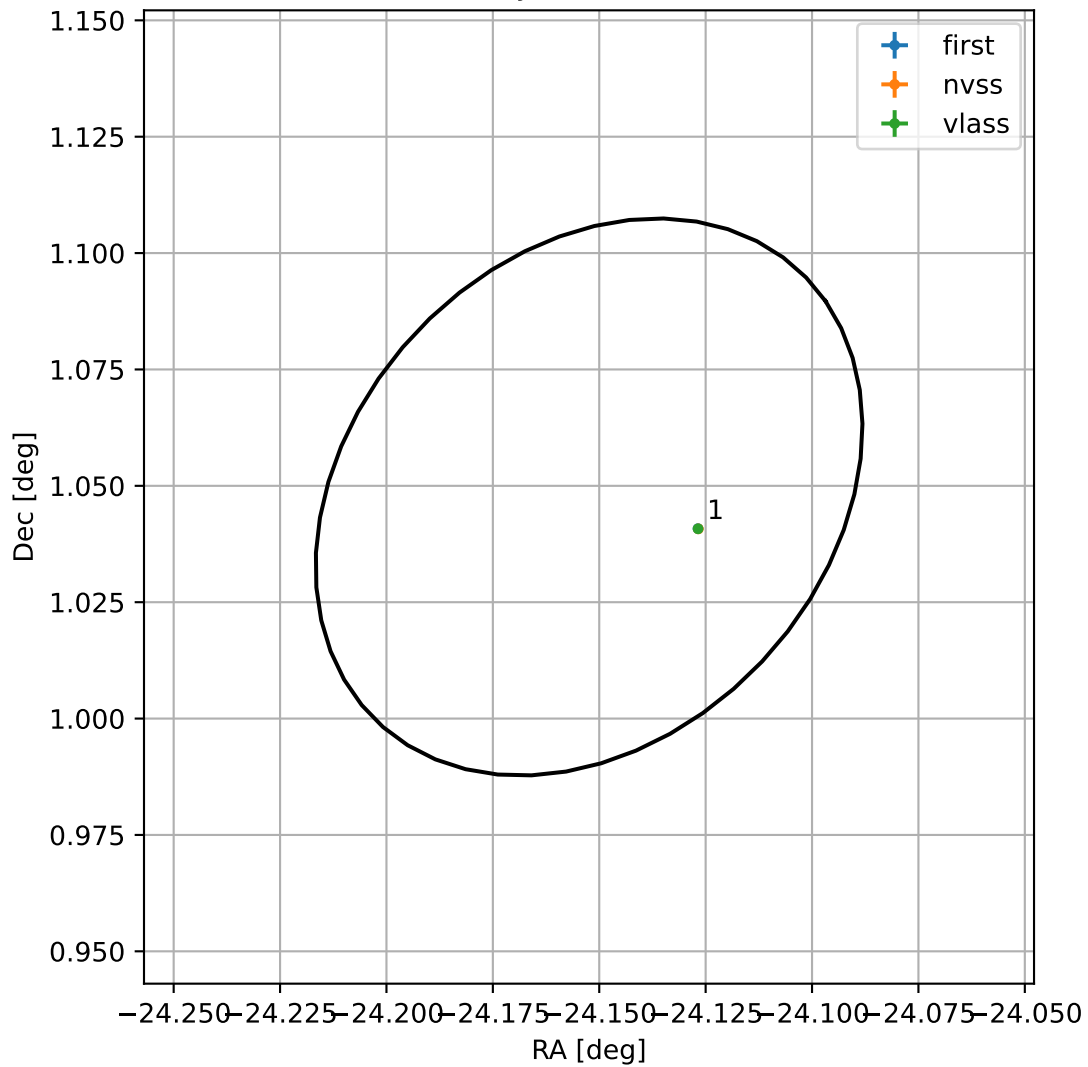
4FGL J2223.3+0102
