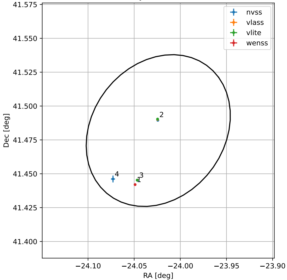
4FGL J2223.9+4128
