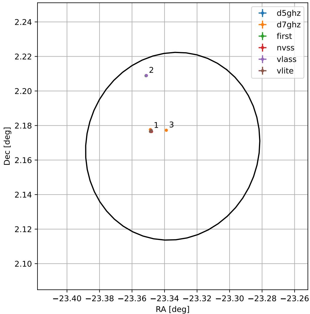
4FGL J2226.6+0210
