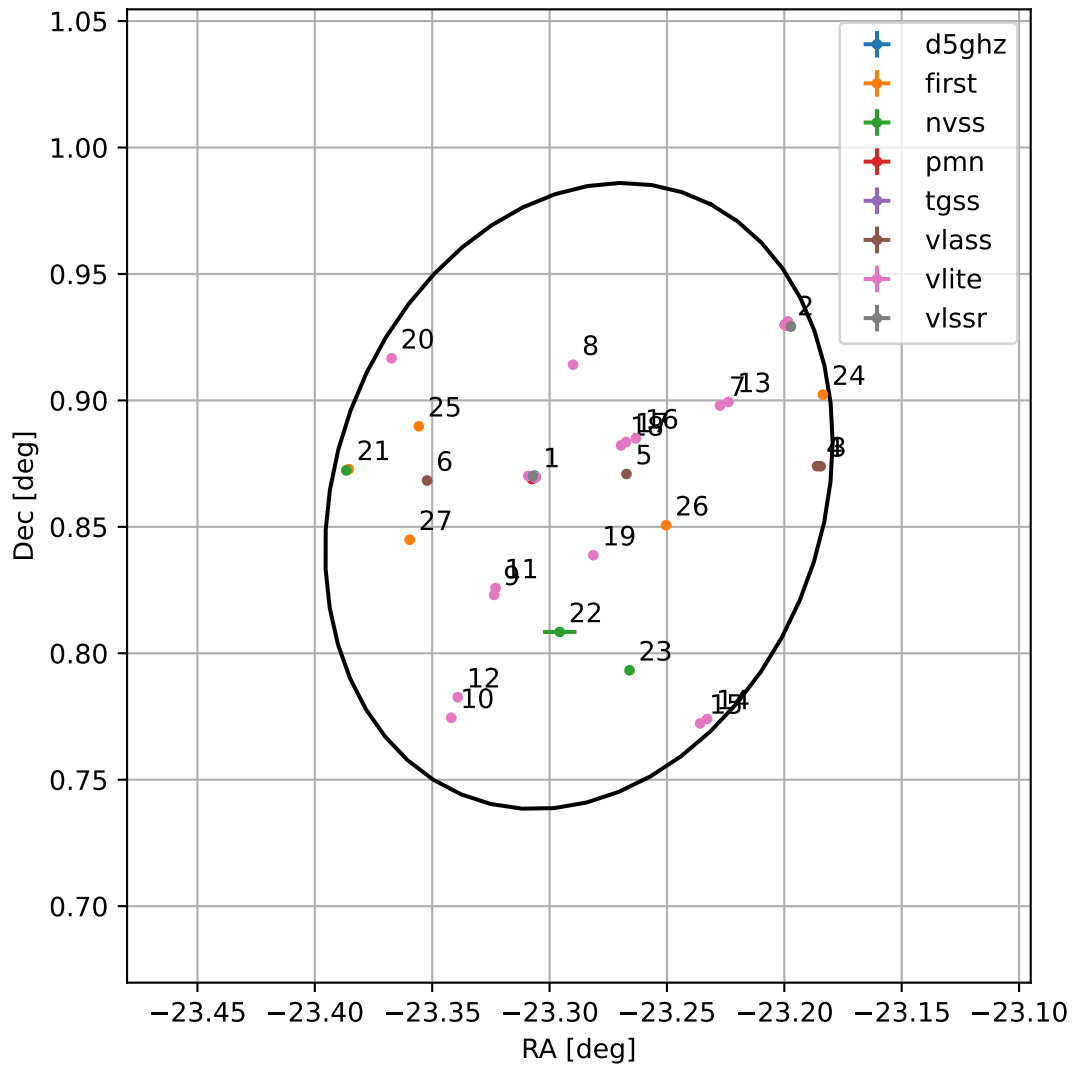
4FGL J2226.8+0051
