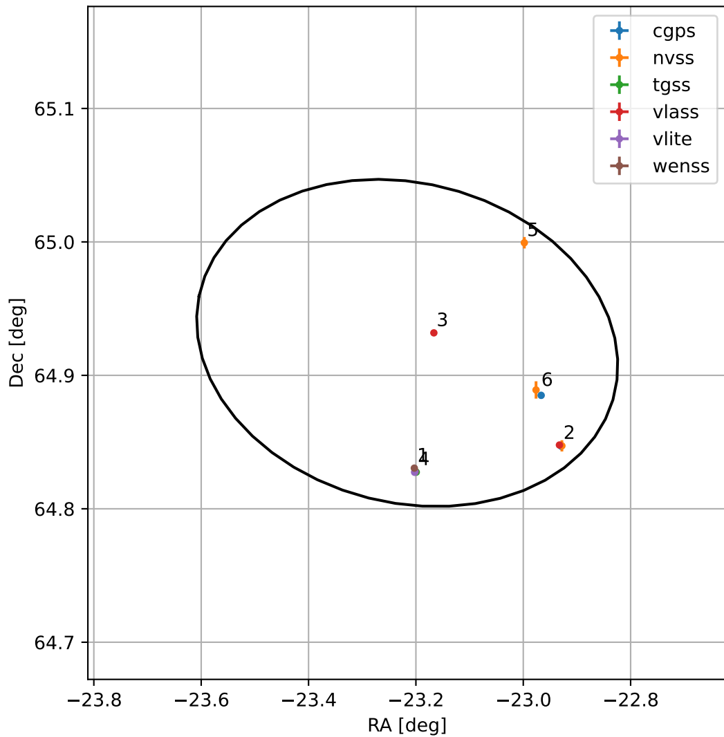
4FGL J2227.1+6455
