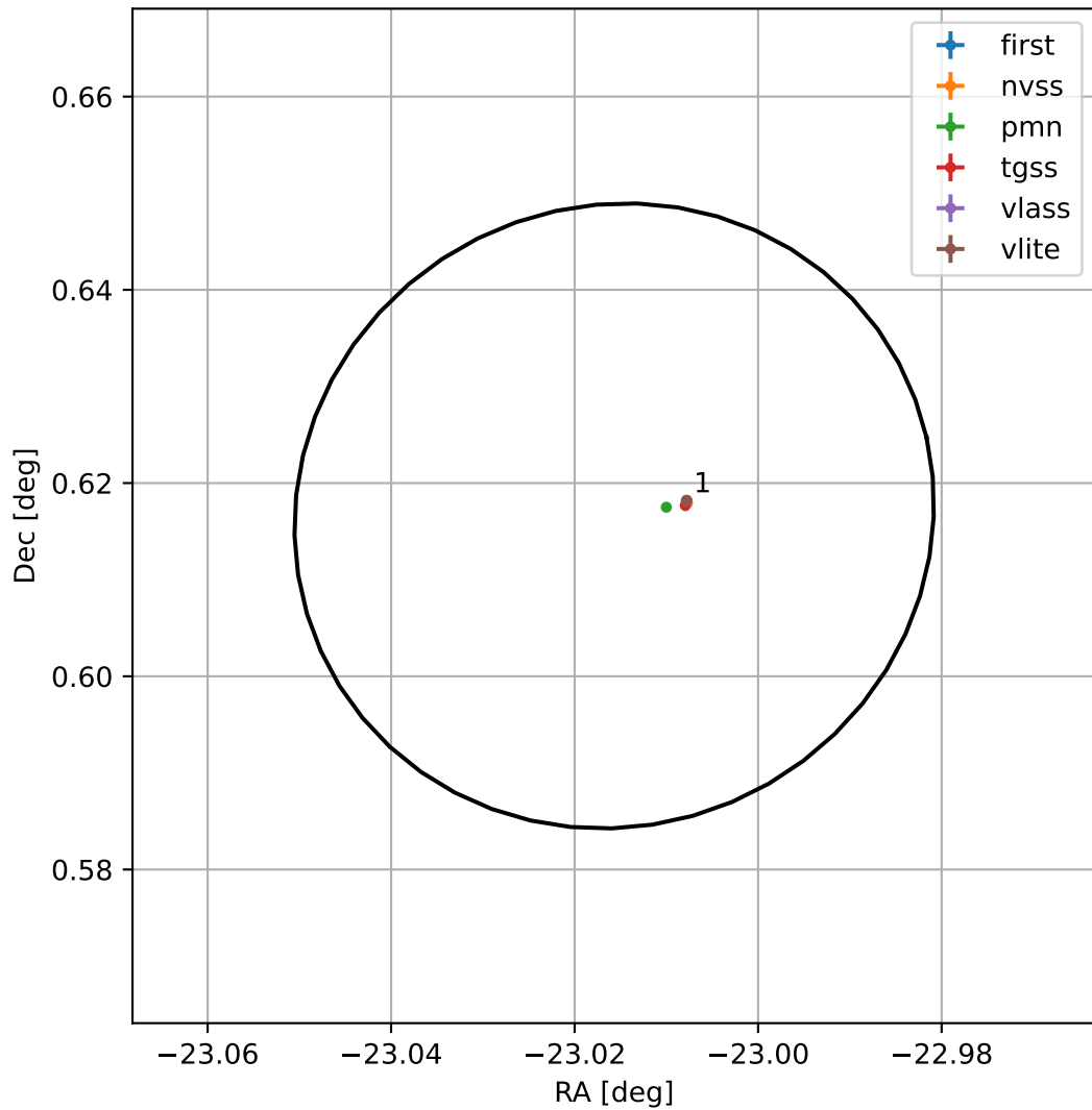
4FGL J2227.9+0036
