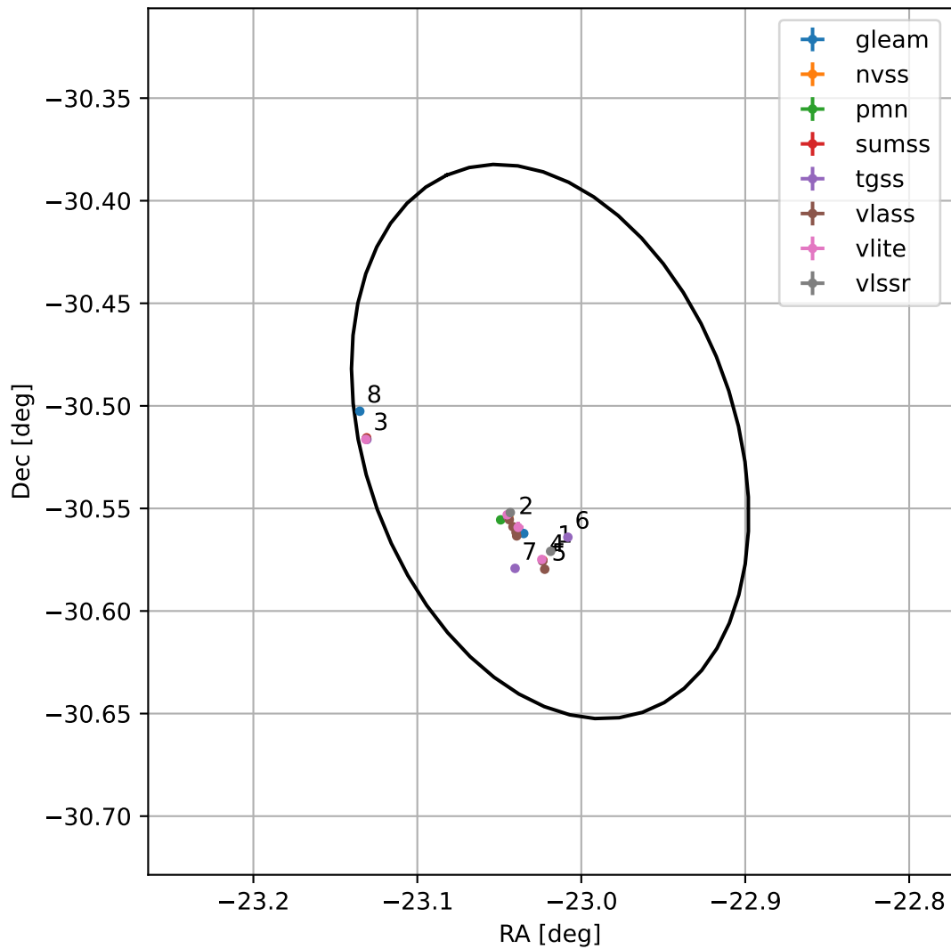
4FGL J2227.9-3031
