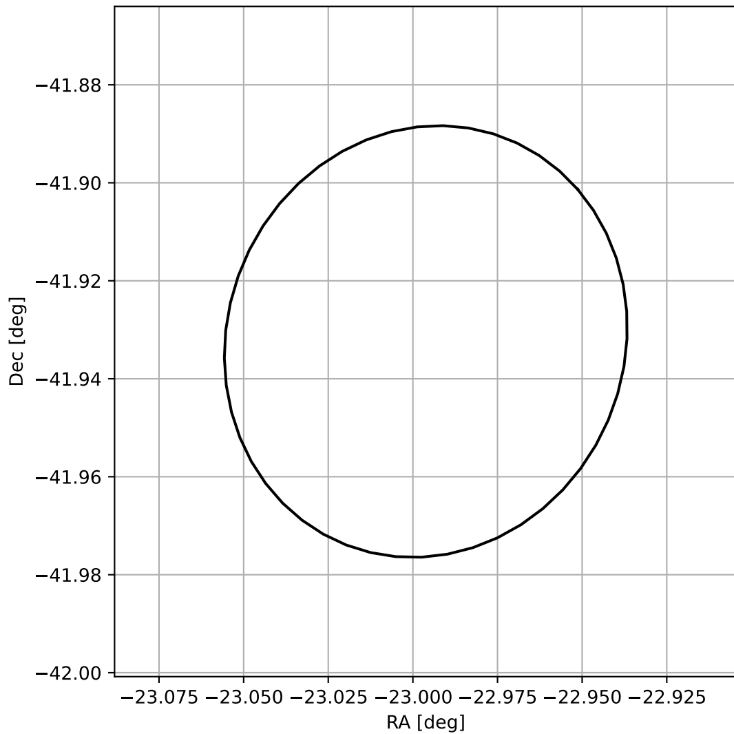
4FGL J2228.0-4155
