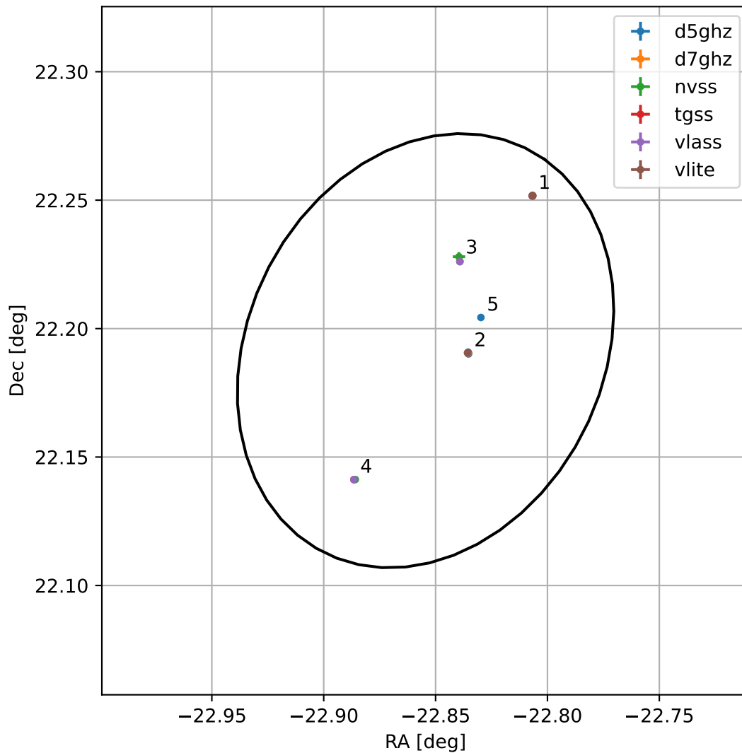
4FGL J2228.5+2211
