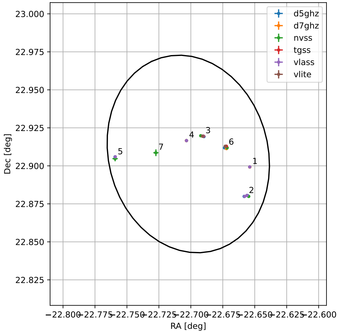
4FGL J2229.1+2254
