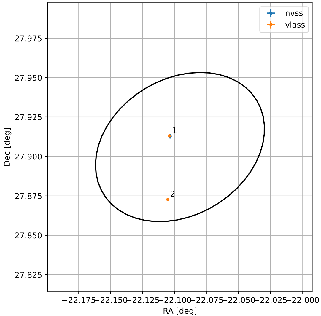
4FGL J2231.6+2754
