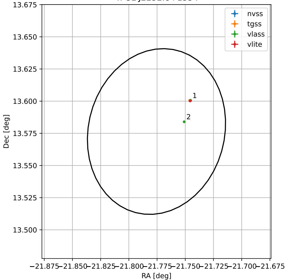
4FGL J2232.8+1334
