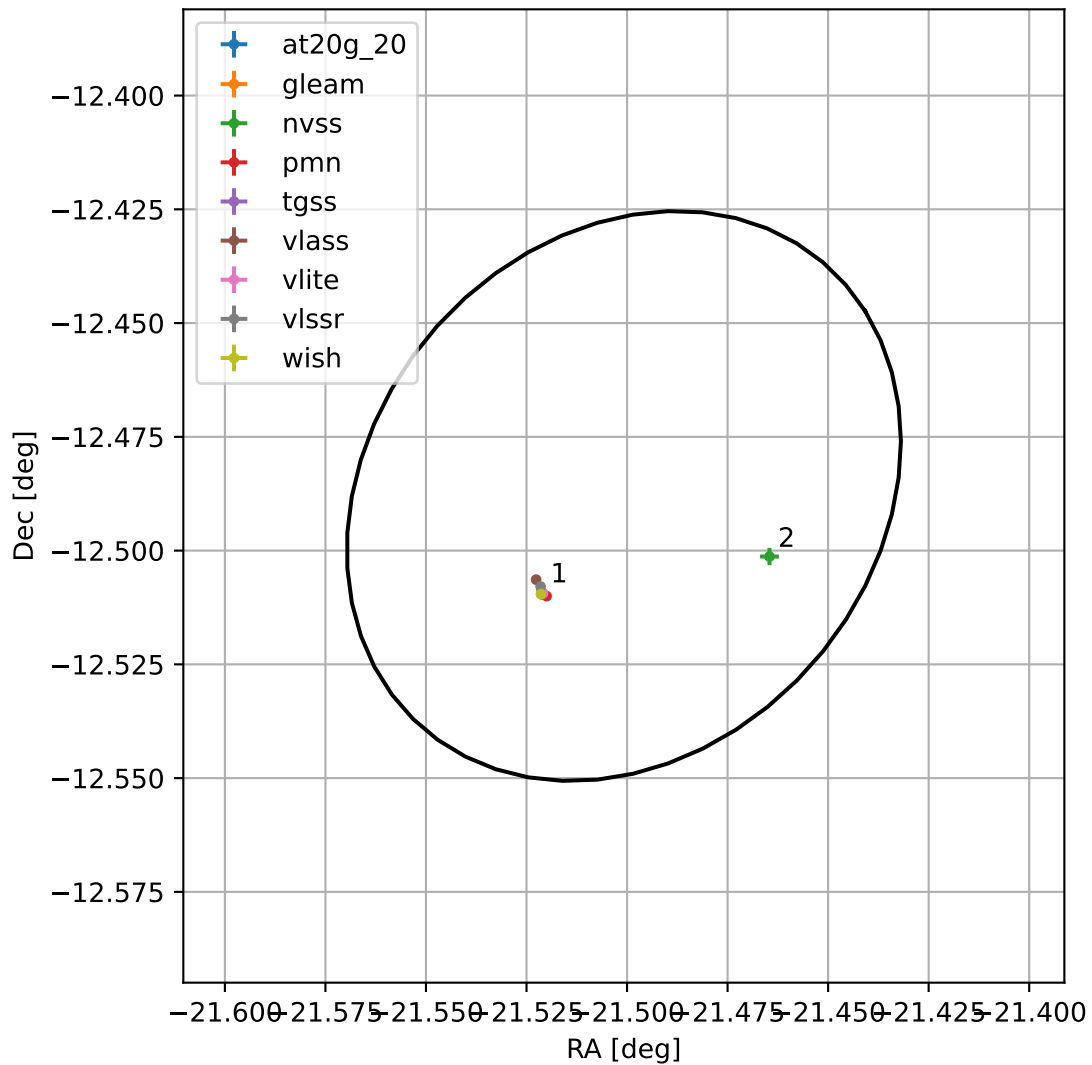
4FGL J2233.9-1229
