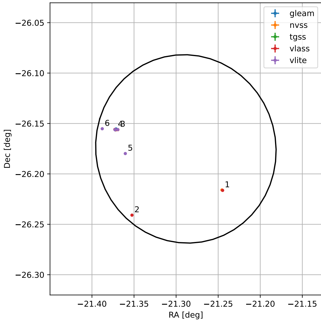
4FGL J2234.8-2610
