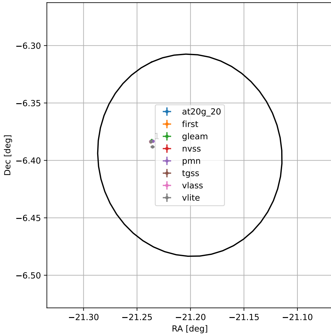
4FGL J2235.1-0623
