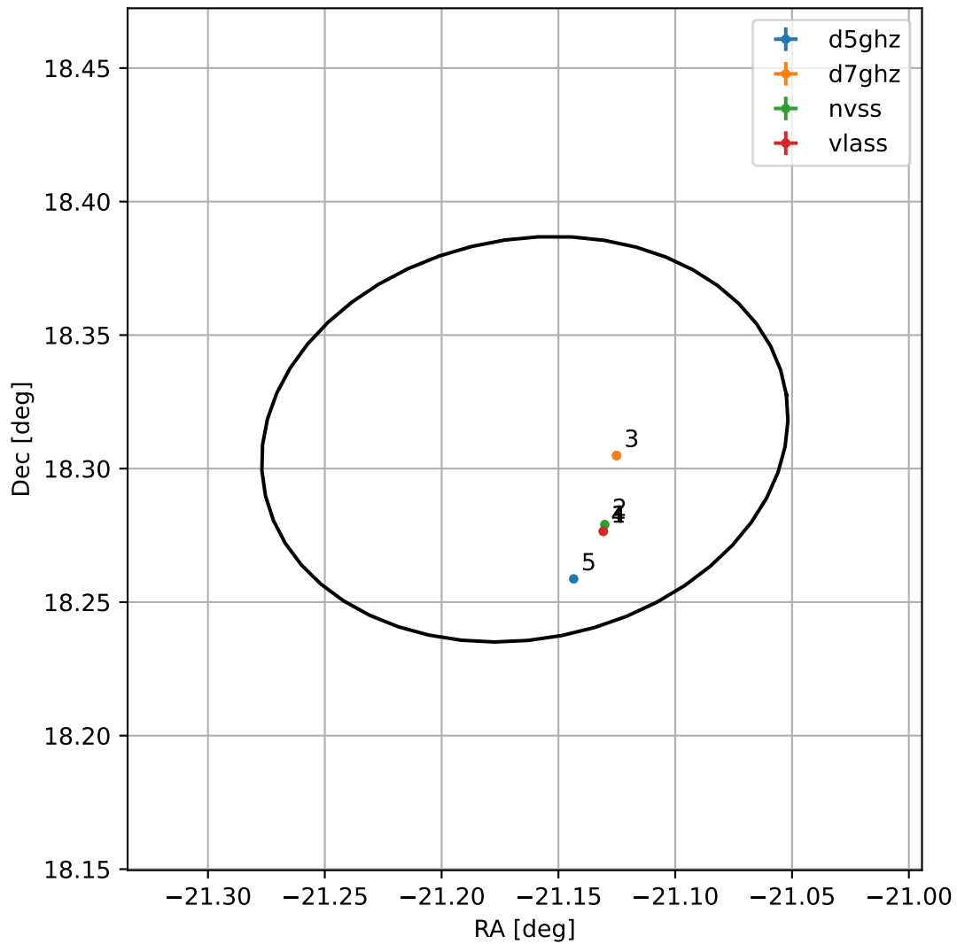
4FGL J2235.3+1818
