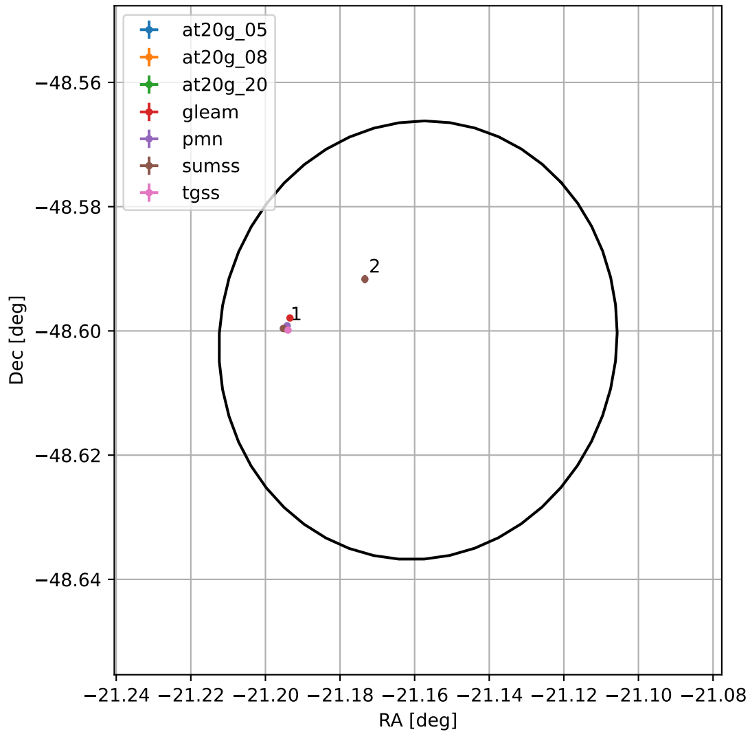
4FGL J2235.3-4836
