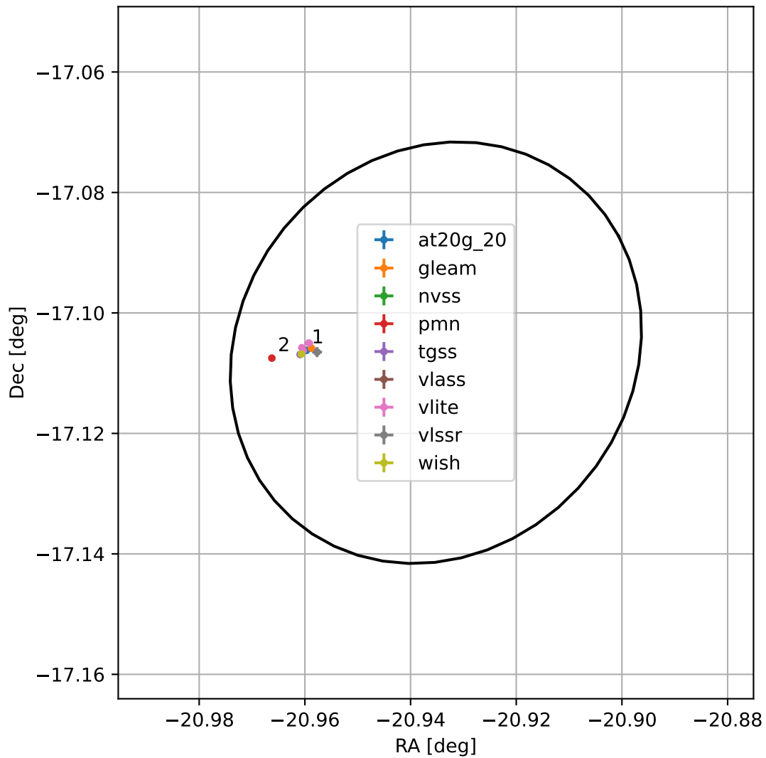
4FGL J2236.2-1706
