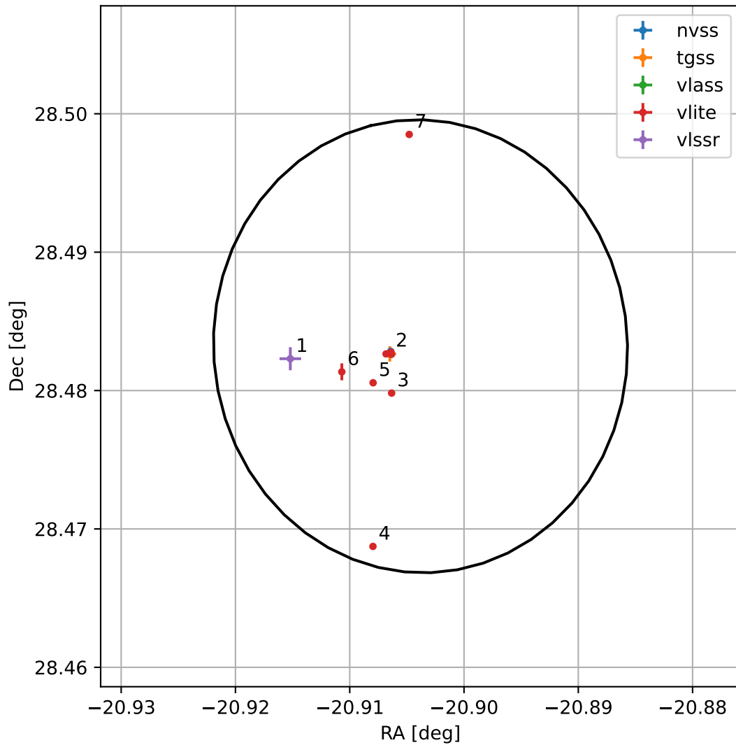
4FGL J2236.3+2828
