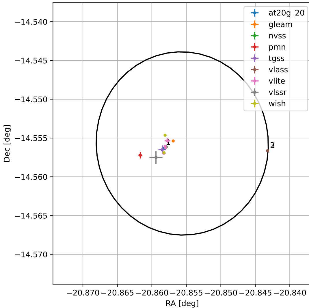
4FGL J2236.5-1433
