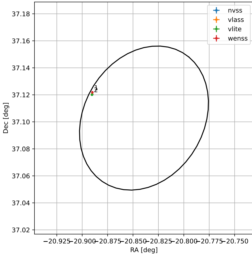
4FGL J2236.6+3706
