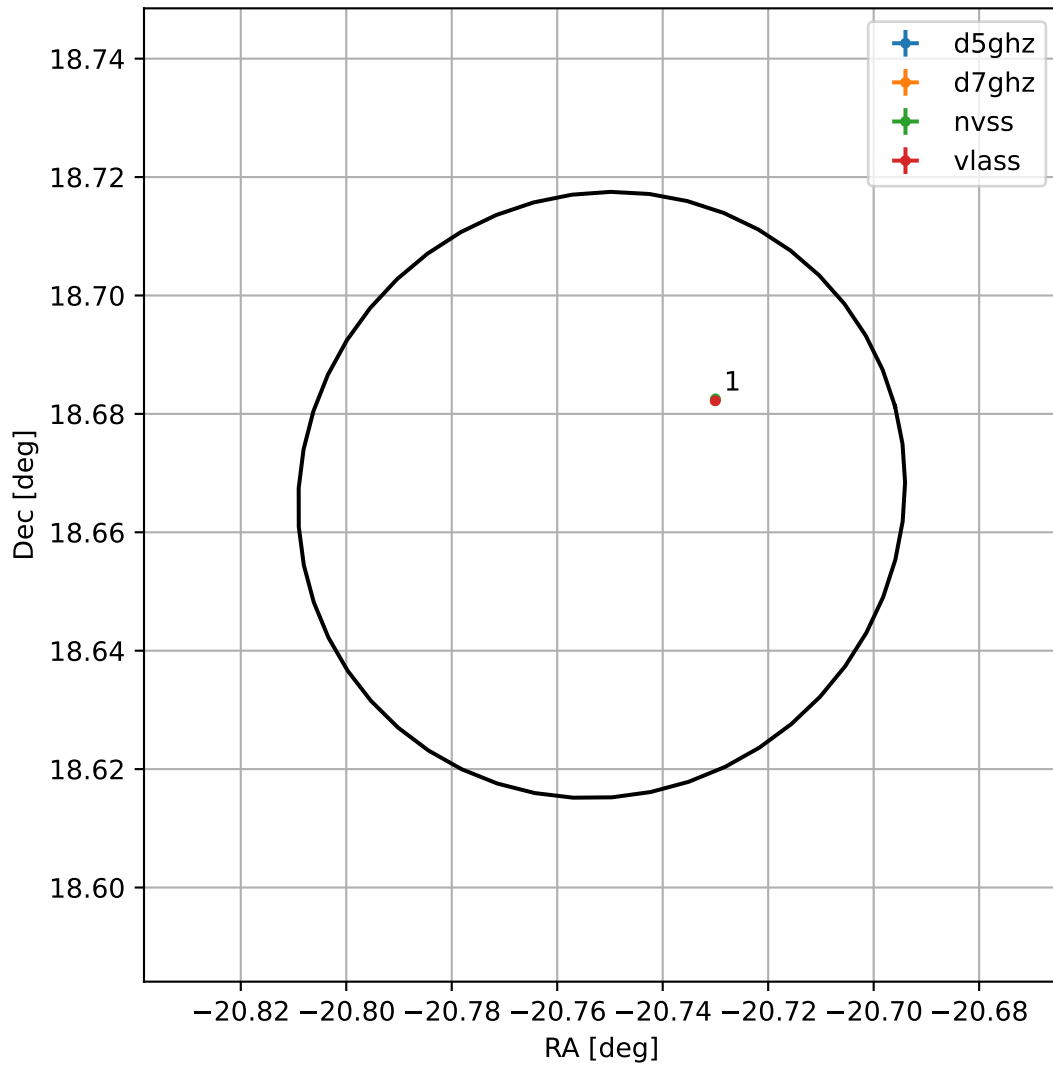
4FGL J2236.9+1839
