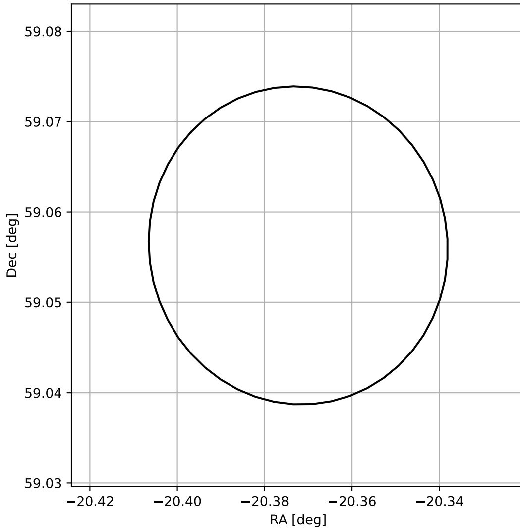
4FGL J2238.5+5903
