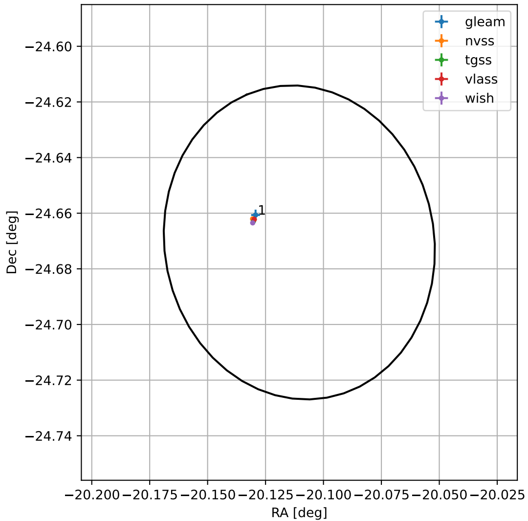
4FGL J2239.5-2440
