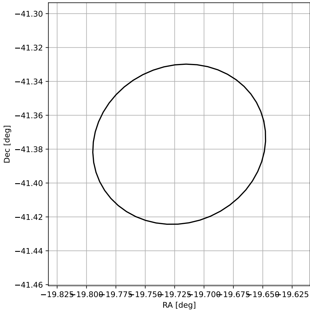
4FGL J2241.1-4122
