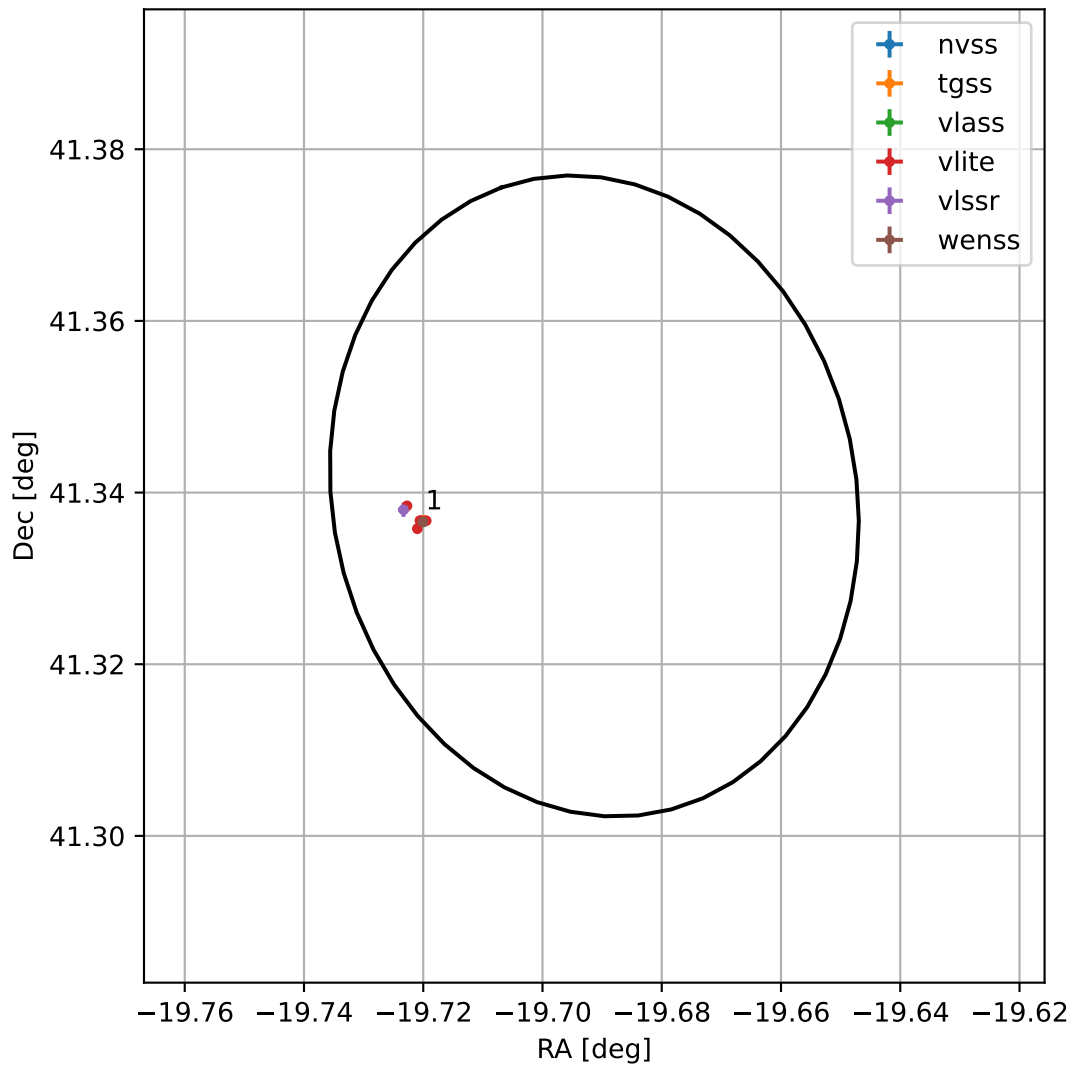
4FGL J2241.2+4120
