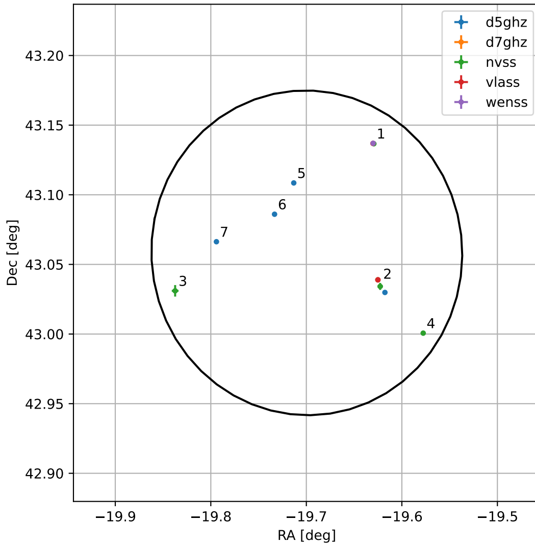
4FGL J2241.2+4303
