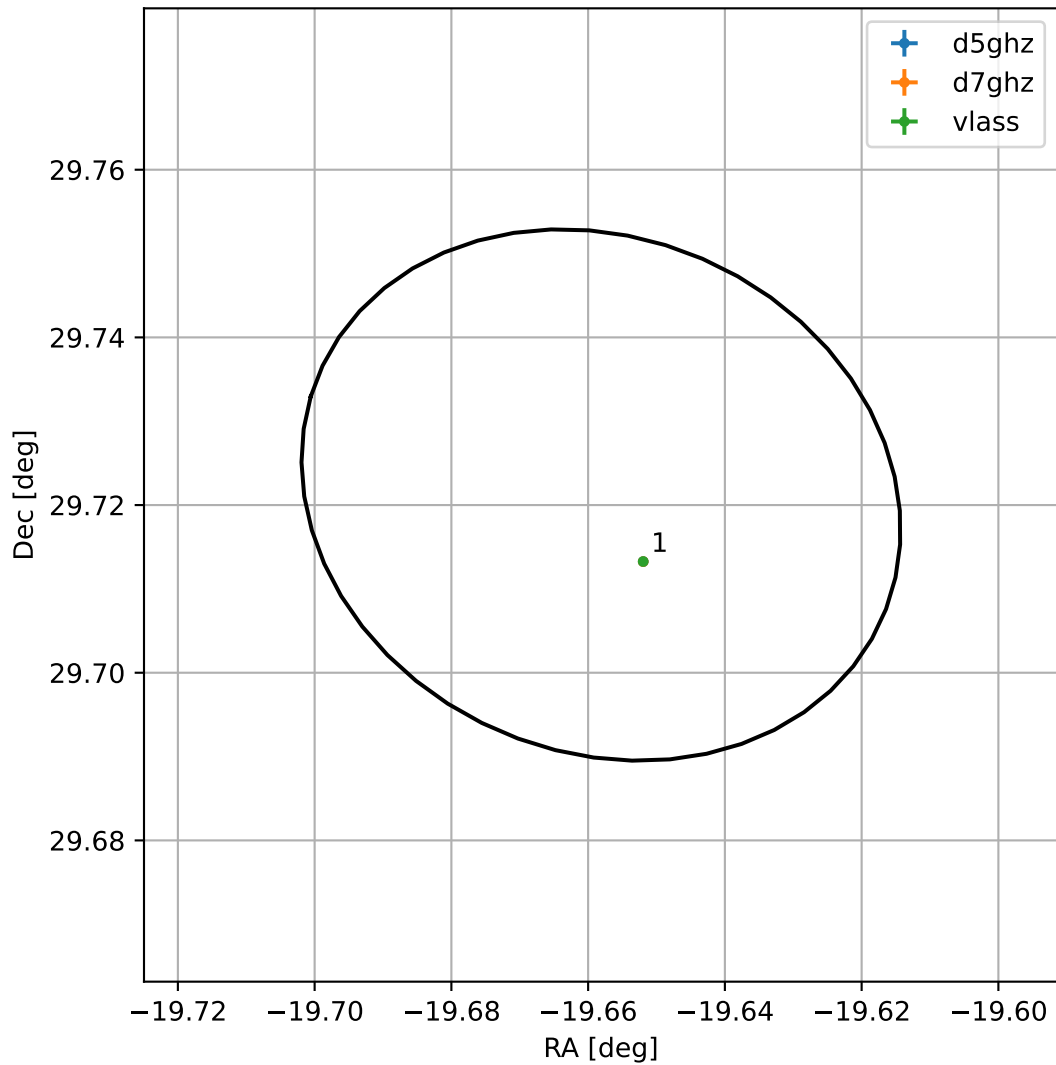
4FGL J2241.3+2943
