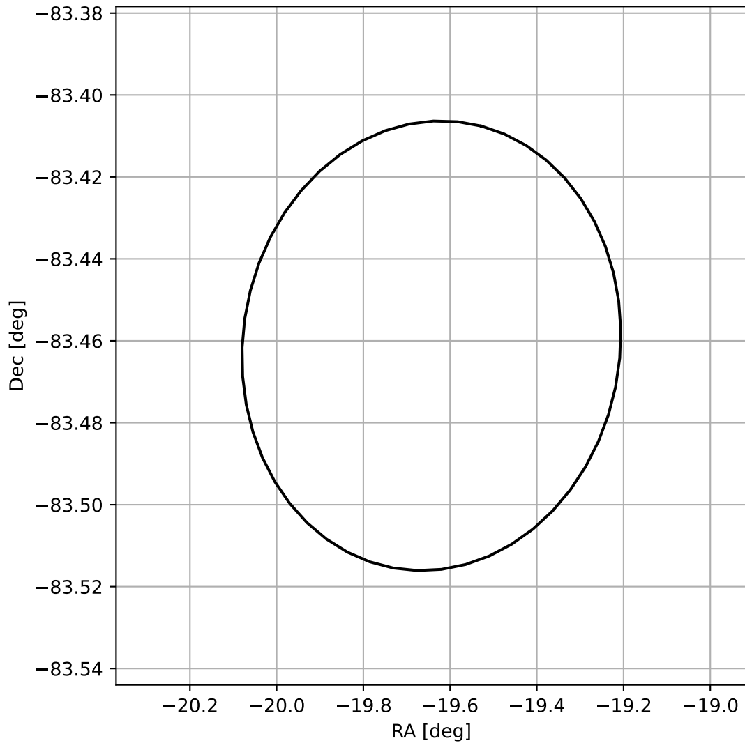
4FGL J2241.4-8327
