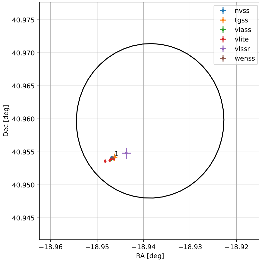
4FGL J2244.2+4057
