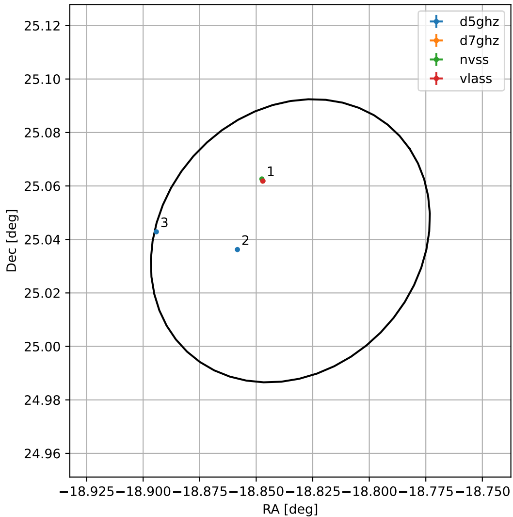
4FGL J2244.6+2502
