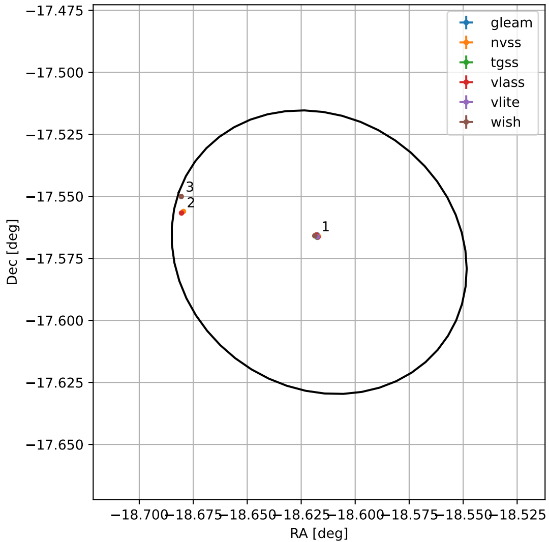
4FGL J2245.5-1734
