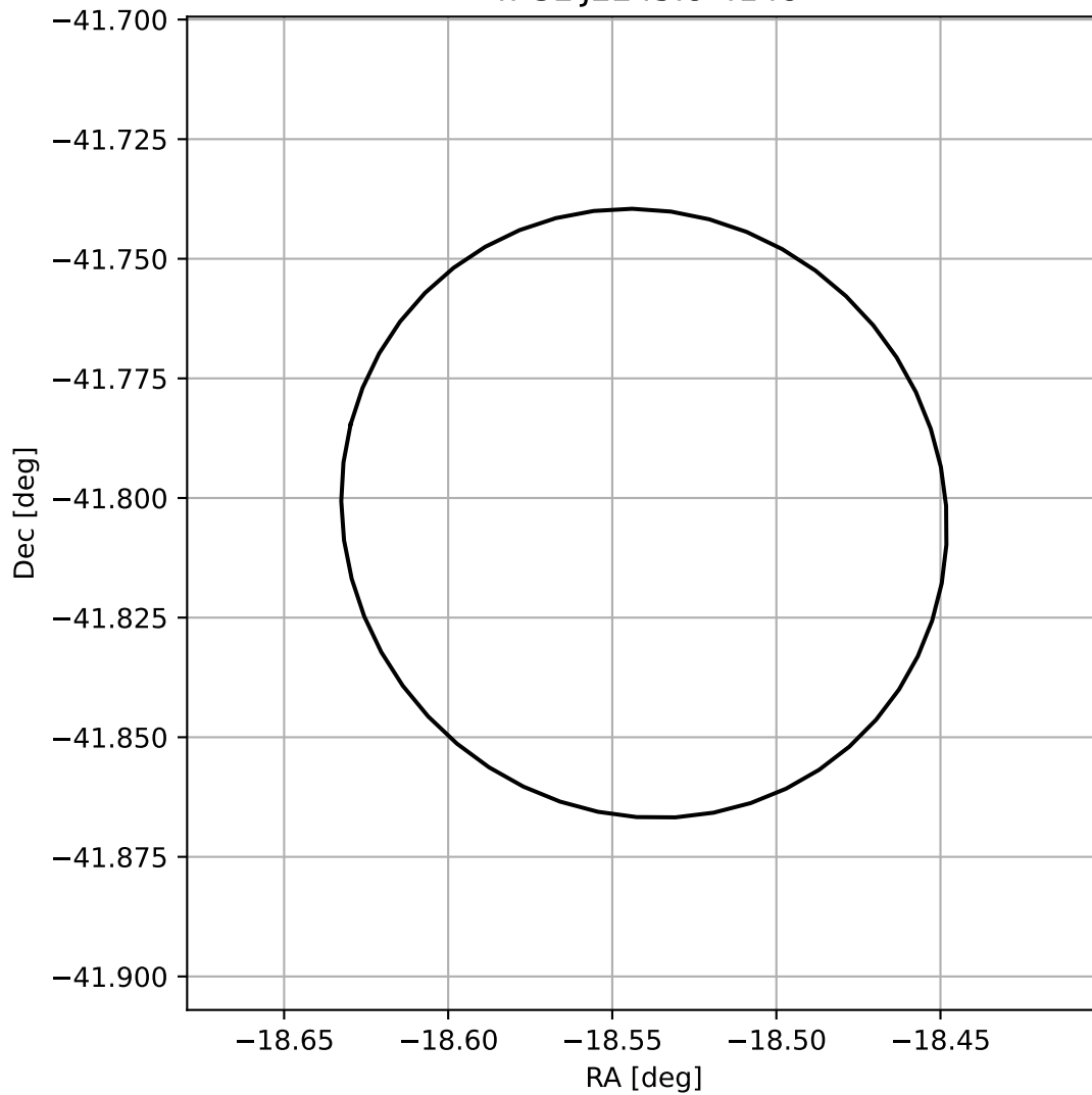
4FGL J2245.8-4148
