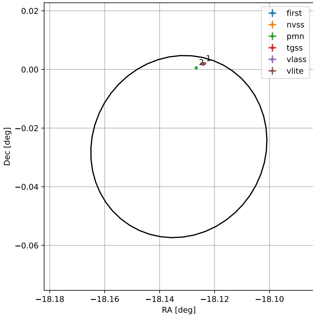
4FGL J2247.4-0001
