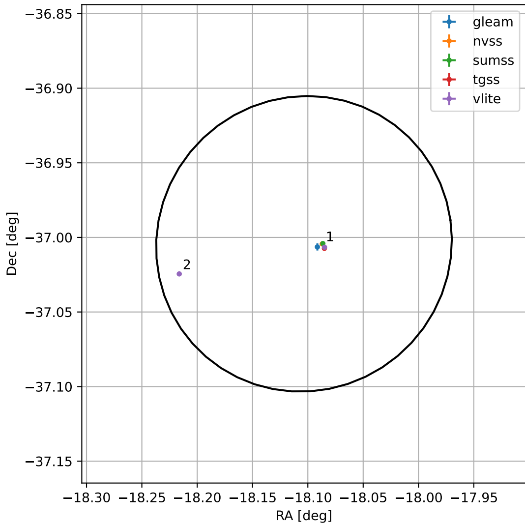
4FGL J2247.5-3700
