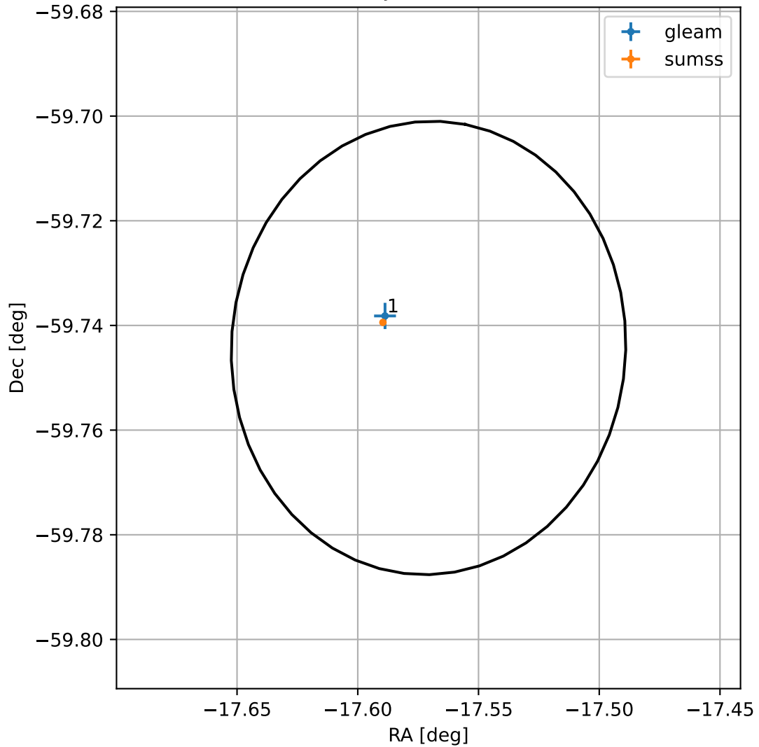
4FGL J2249.7-5944
