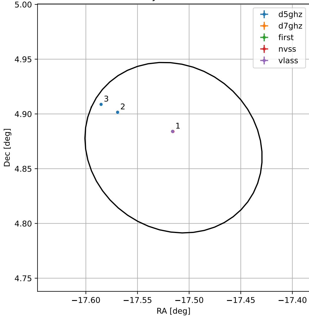
4FGL J2249.9+0452
