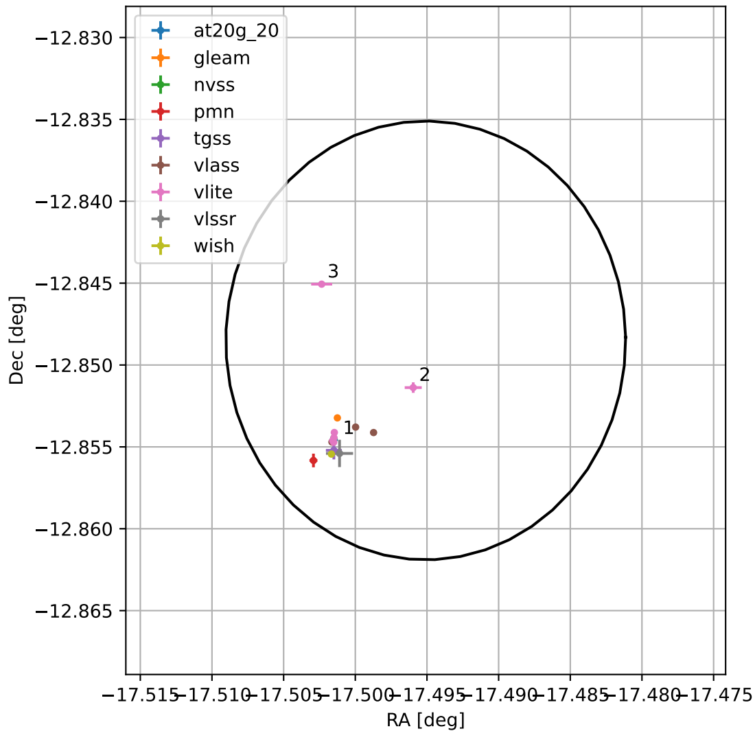
4FGL J2250.0-1250
