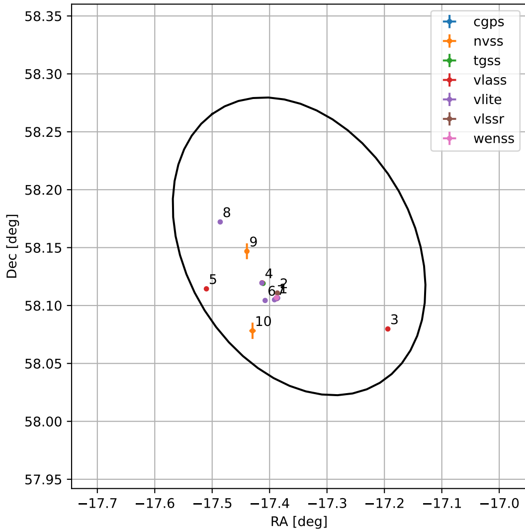
4FGL J2250.6+5809
