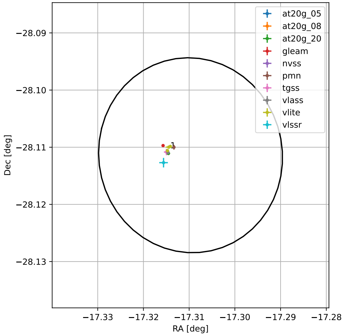
4FGL J2250.7-2806
