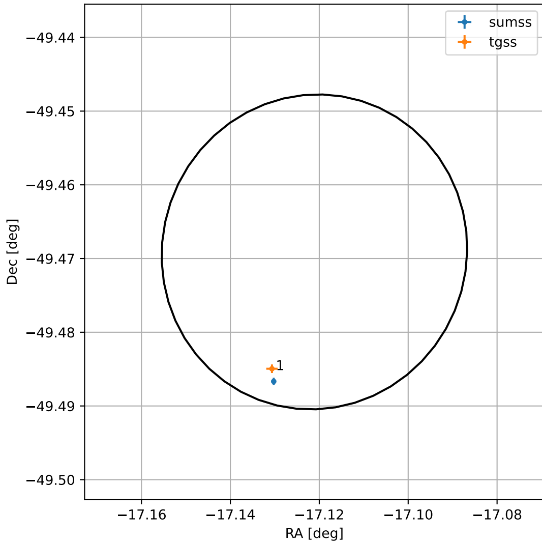
4FGL J2251.5-4928
