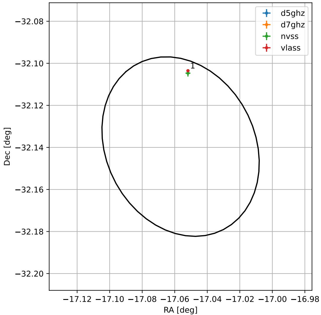
4FGL J2251.7-3208
