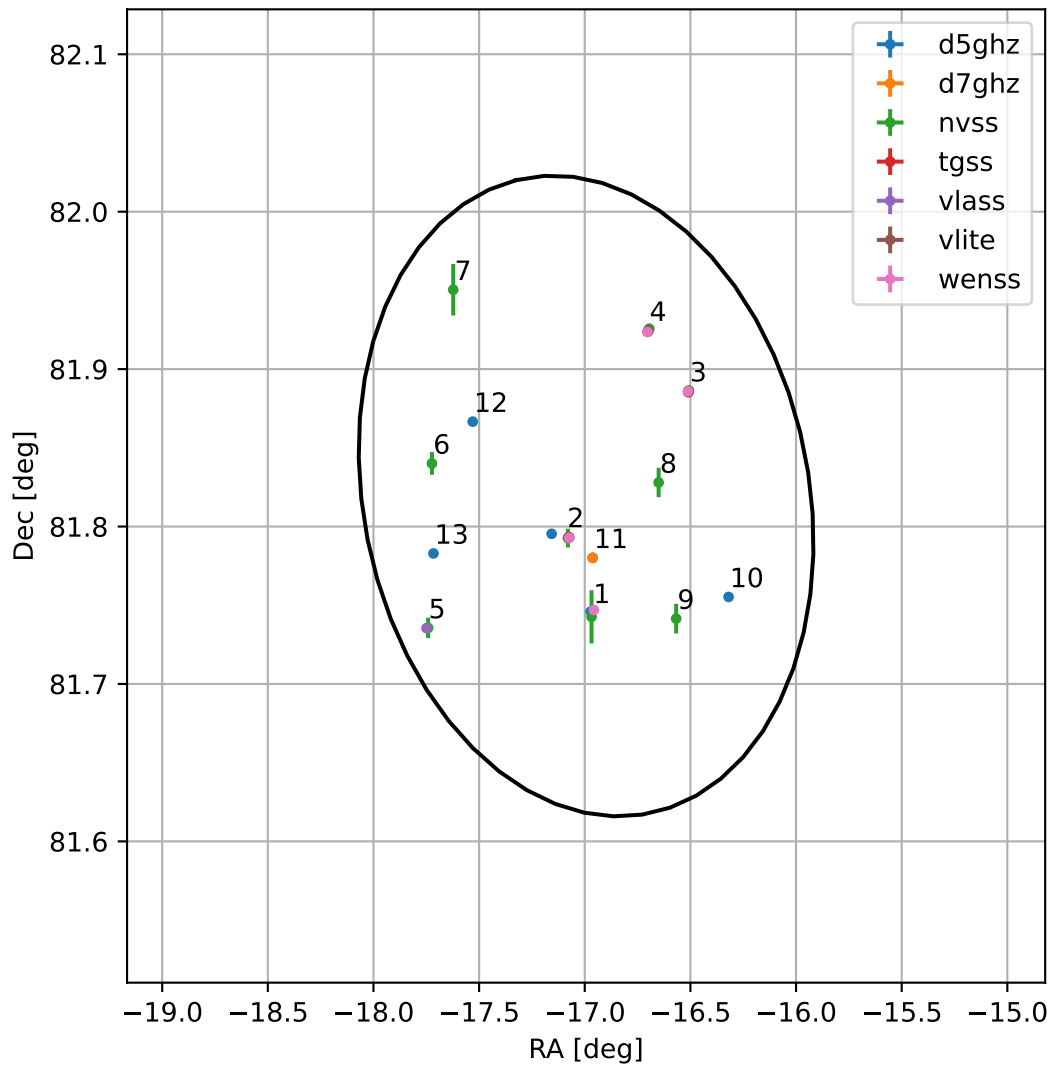
4FGL J2252.0+8149
