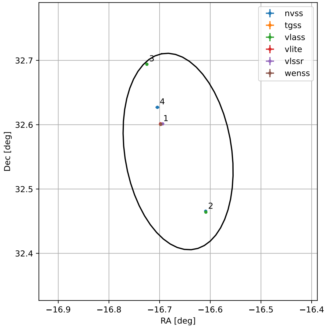
4FGL J2253.3+3233
