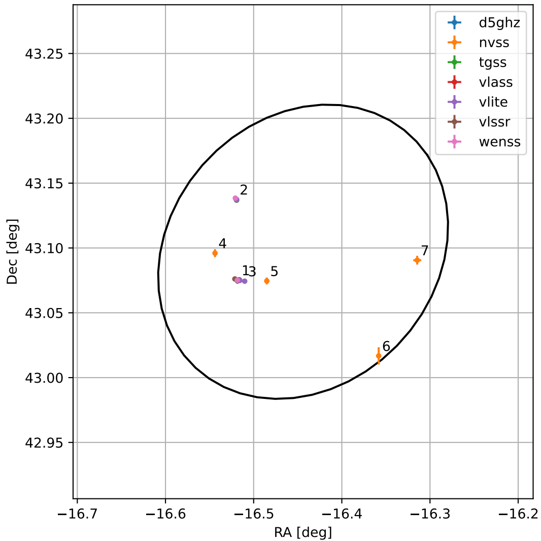
4FGL J2254.2+4305
