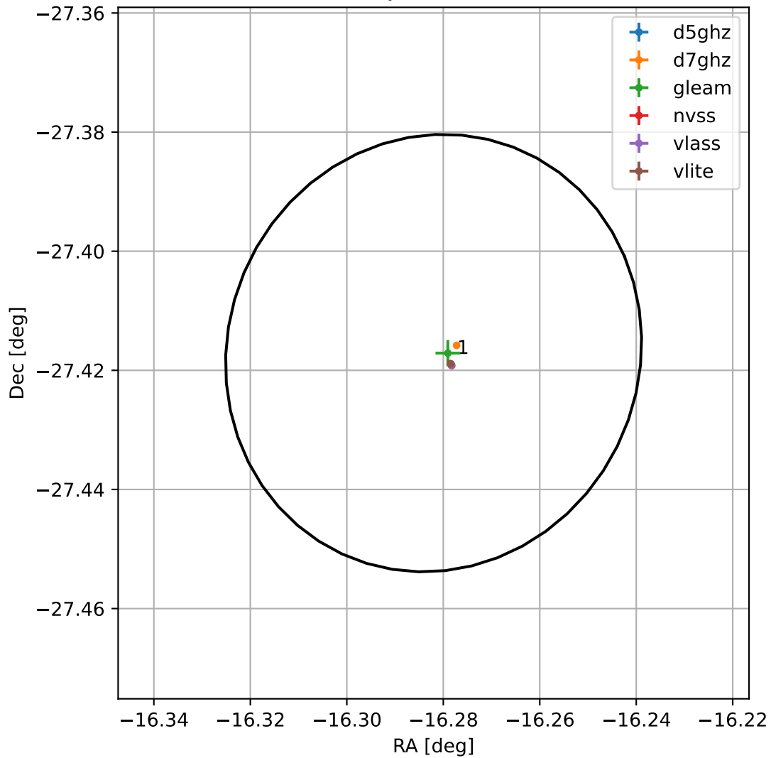
4FGL J2254.8-2725
