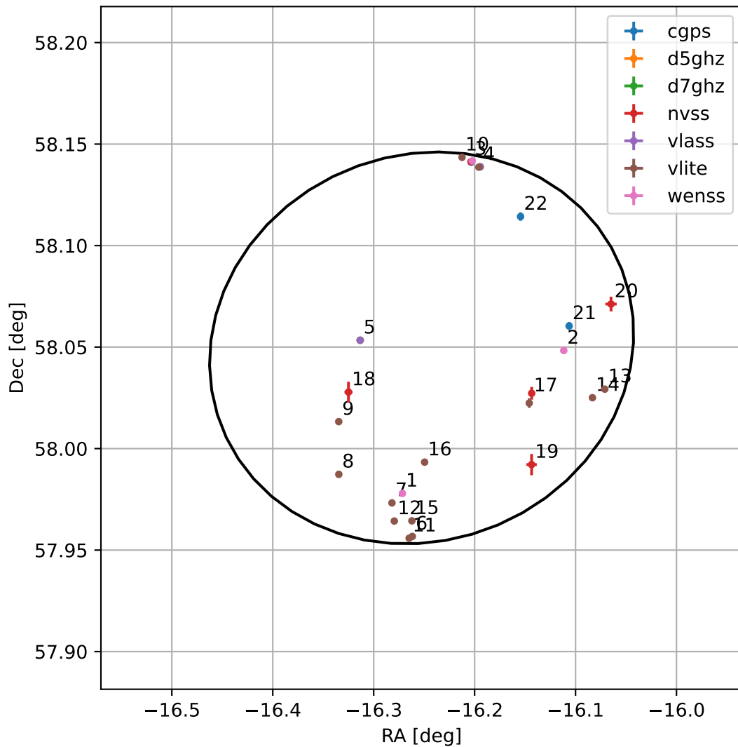
4FGL J2254.9+5802
