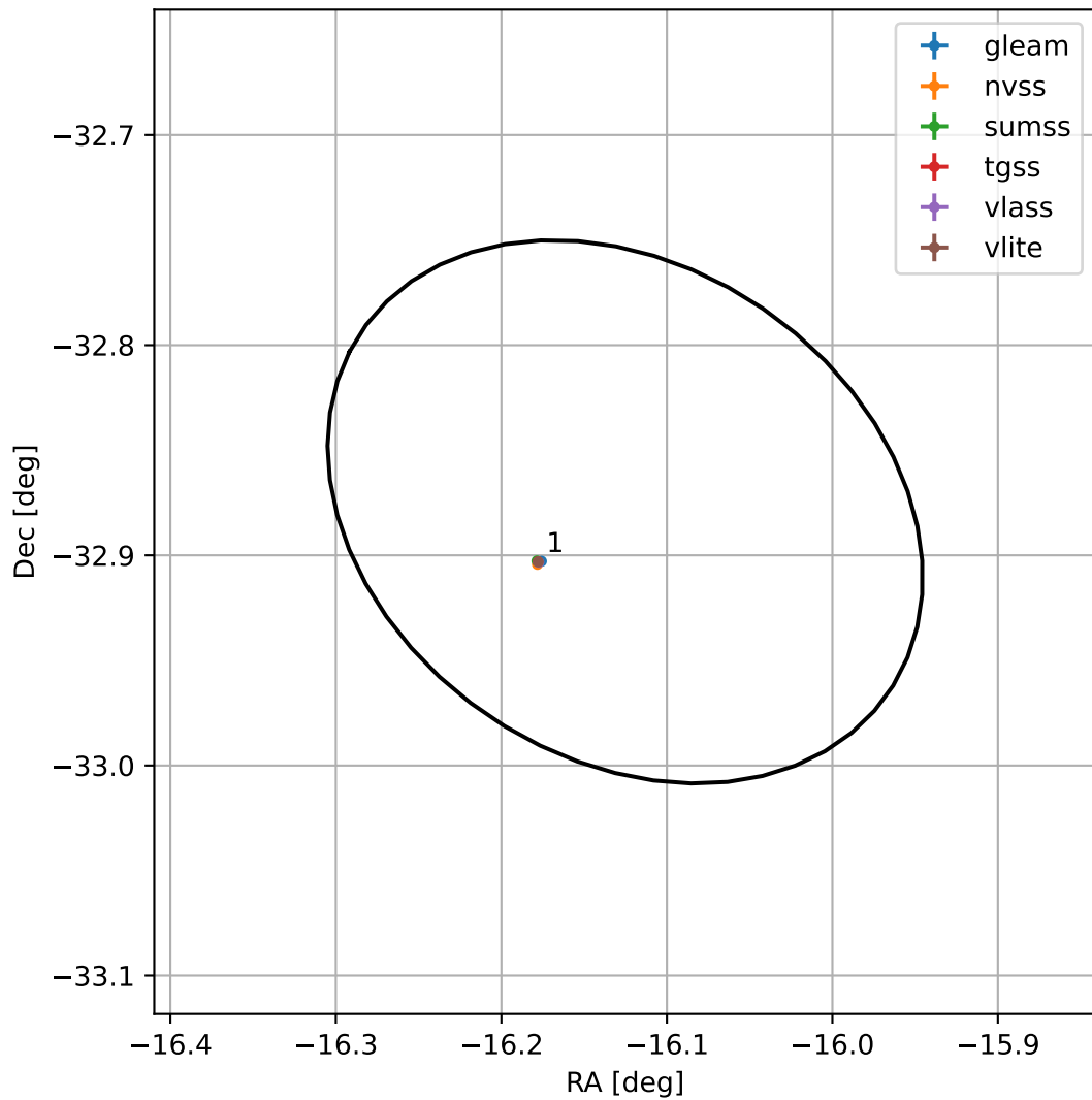
4FGL J2255.4-3252
